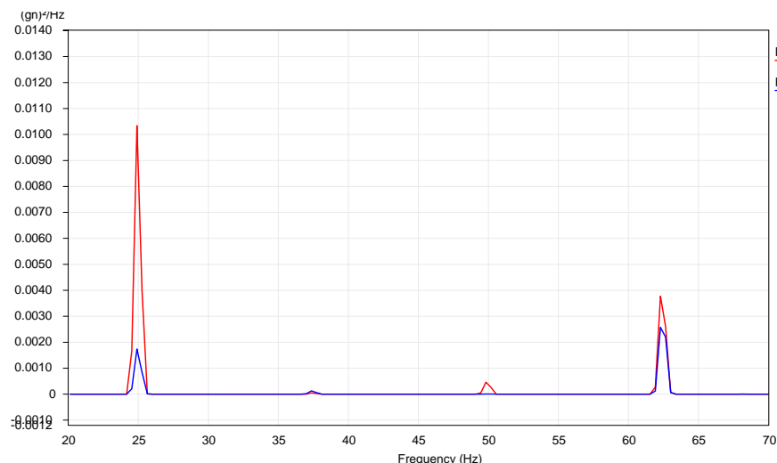
Figure 2 Power spectrum of the diesel generator acceleration measured at one of the mounting feet, before (red) and after (blue) the tuned absorbers installation
