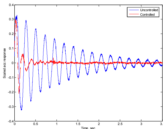
Figure 2 Accelerations of the mounted mass isolated by an uncontrolled (blue/solid line) and controlled (red/dashed line) air mount
