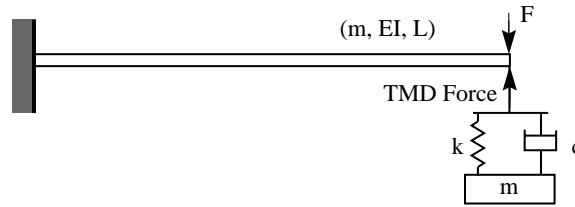
Figure 1 A tuned mass damper appended to a structure
