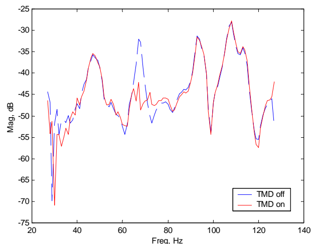
Figure 3 FRFs mapping the shaker voltage to the pressure
